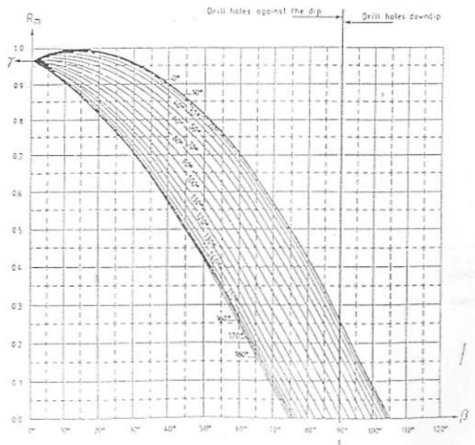
Diagram 4. \alpha = 75^\circ
