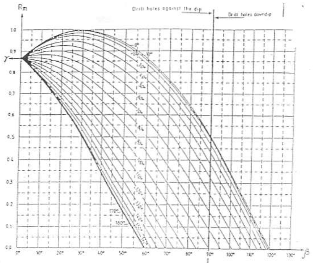
Diagram 3. \alpha = 60^\circ
