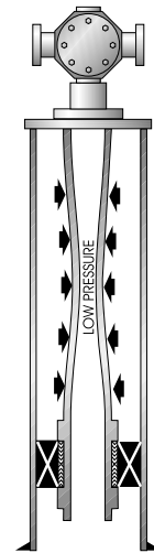
Reverse Ballooning
