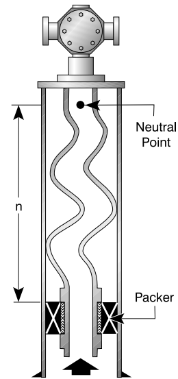
Buckled Tubing
