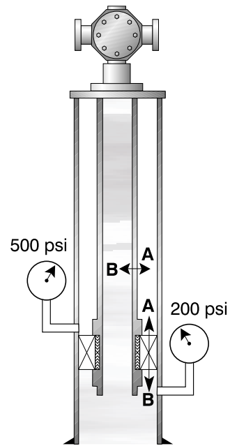
Differential Across Tubing Differential Across Packer
