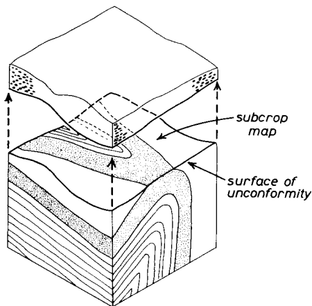
Fig. 5.5 The concept of the subcrop map.
