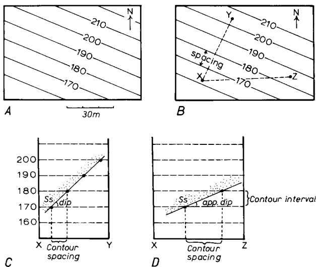
Fig. 2.14 Drawing sections.
