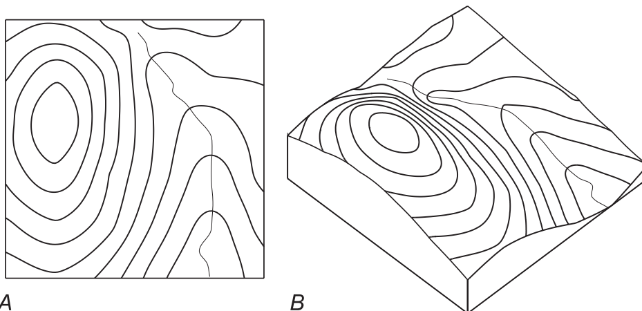
Fig. 2.12 Contour patterns and the form of a surface.
