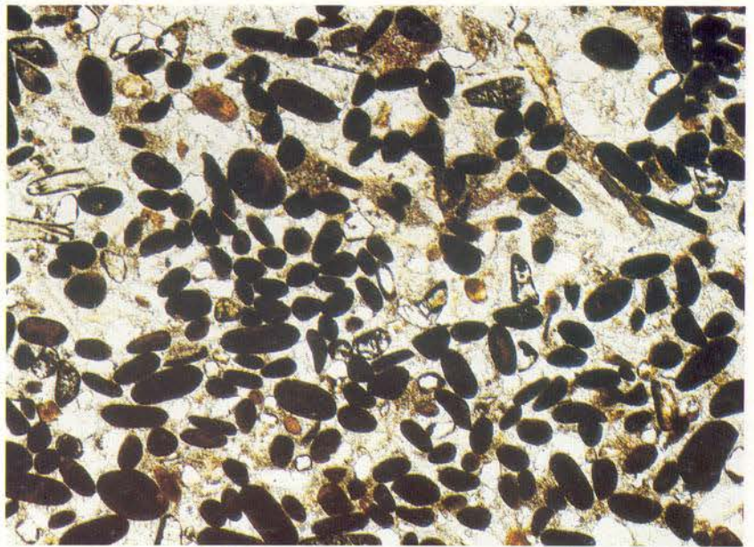
173: Northampton Sand Ironstone, Middle Jurassic, Northamptonshire, England; magnification \times 37 , PPL. 174: Frodingham Ironstone, Lower Jurassic, Scunthorpe, England; magnification \times 35 , PPL.
